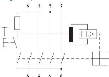
Wiring diagram
