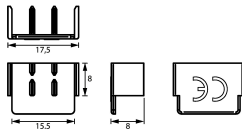
Dimensional drawing Group view
